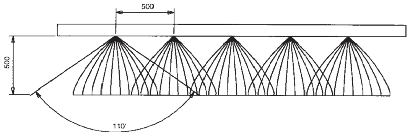
Above: Optimal nozzle spacing and spray height with a nozzle fan angle of 110 degrees.
